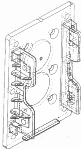
Eclipse 2" x 3-1/2" STD Rail Top and Bottom Stair Bracket (Also used for T-Rail Stair Bottom Rail)
