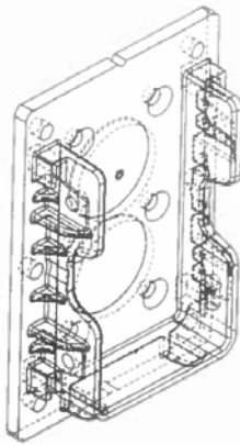
Eclipse 2" x 3-1/2" STD Top and Bottom Rail Straight Bracket
