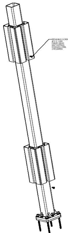
FIGURE 10– STEEL POST MOUNT TOWER
