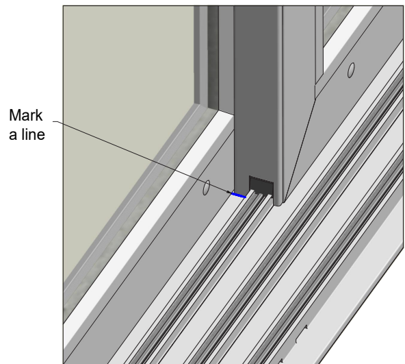
DWG 30
