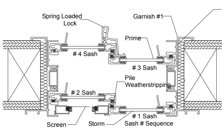
3376 Vertical Section
