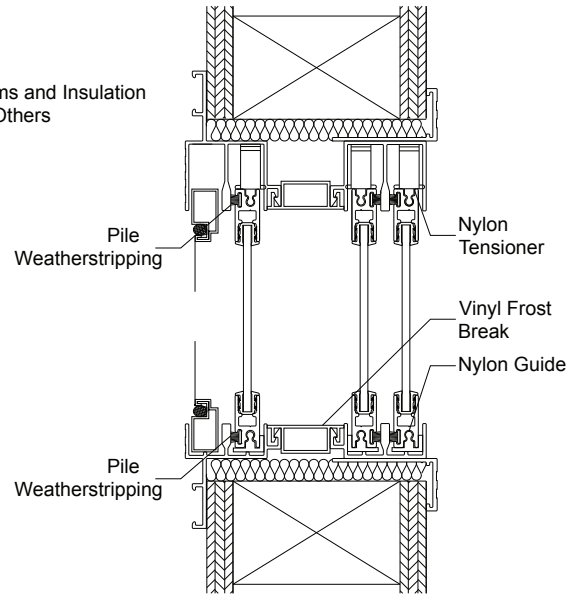
3376 Horizontal Section
