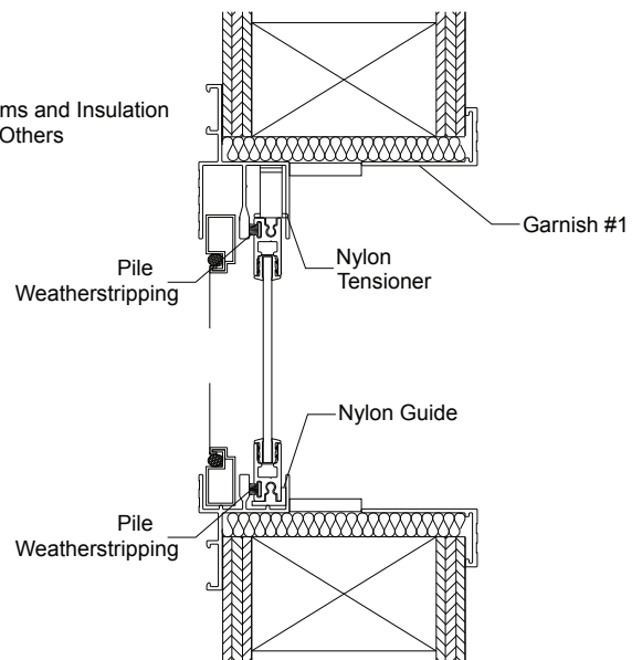
Mark IV Horizontal Section
