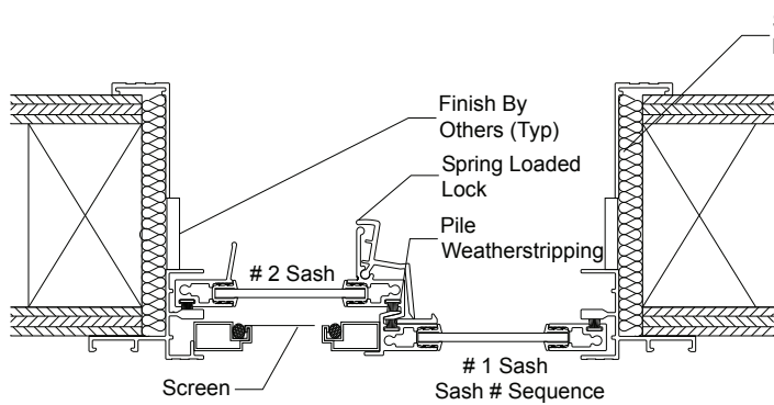
Mark IV Vertical Section
