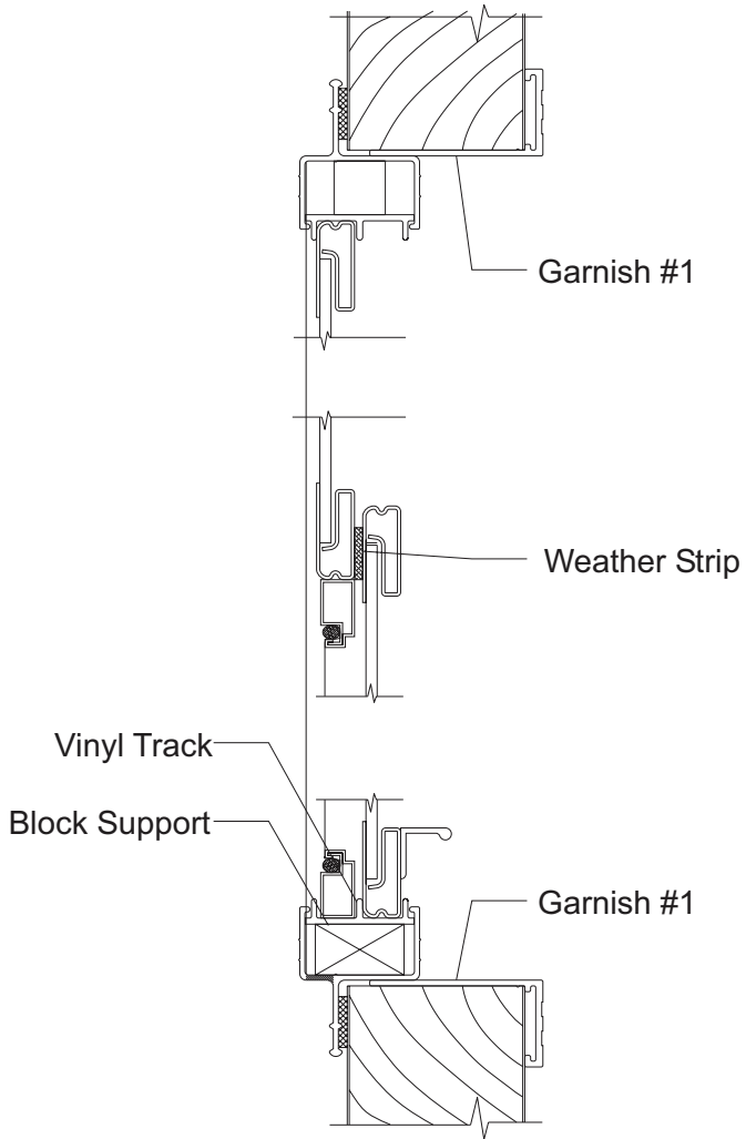
8000 Vertical Section
