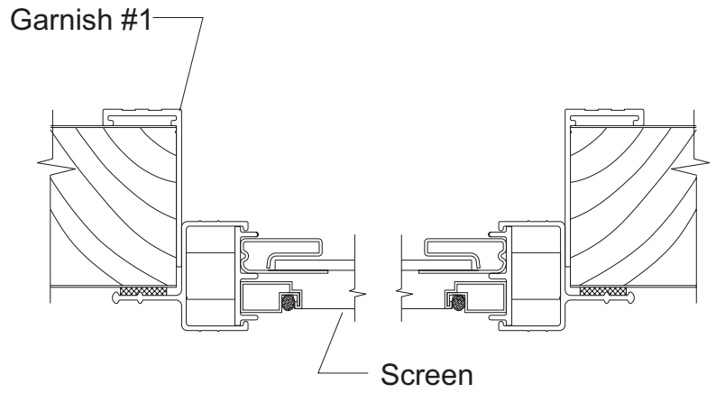
8000 Horizontal Section
